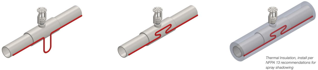
FIGURE 1: SPRINKLER HEAD WITHOUT SPRIG
