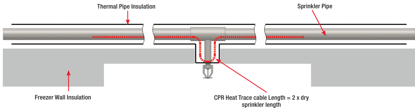
FIGURE 3: DRY PENDANT SPRINKLER IN FREEZERS
